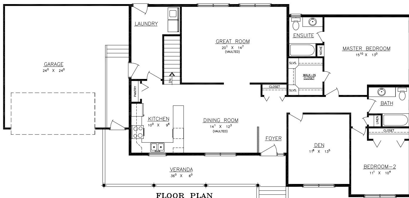
FLOOR PLAN
